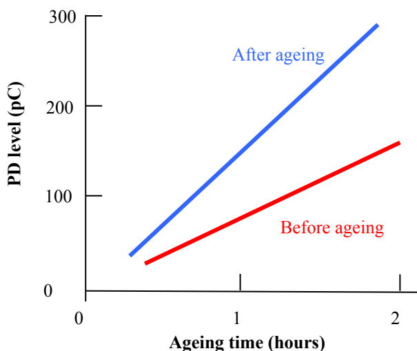
Figure 1 PD activity in PE as a function of time before and after ageing
